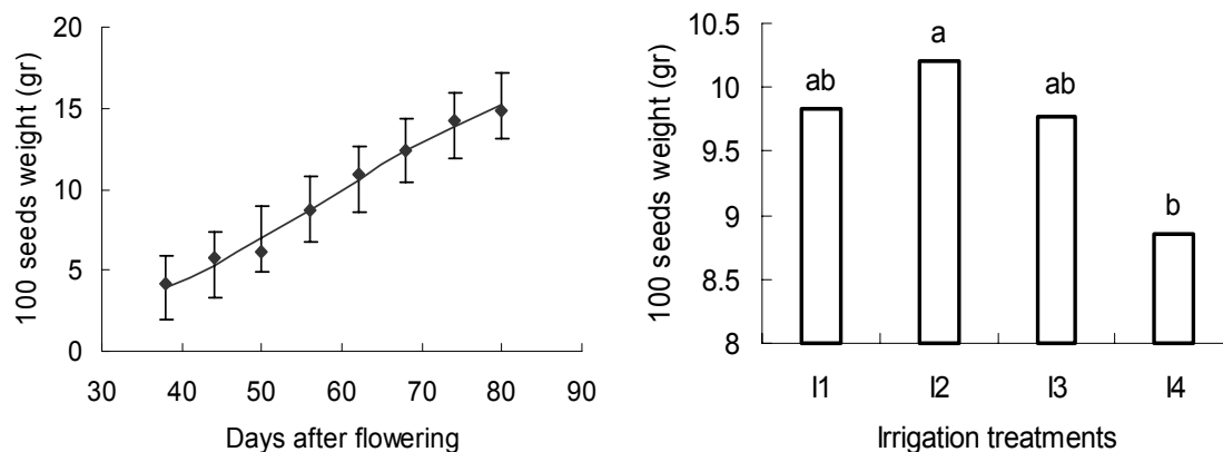
Fig. 2. Logistic regression relationship between observed and predicted values of 100 seed weights ( Y = \frac{0.39 \times 18.7}{0.39 + (18.71 - 0.39) \text{EXP}(-0.066x)} , R^2=0.99 ) (left). 100 seed weights change in different irrigation treatments (right).
