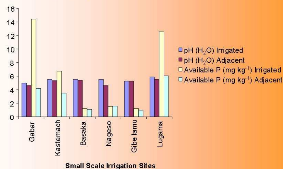
Fig. 3. Soil pH and available P in irrigated and adjacent non-irrigated farmlands
