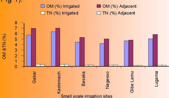
Fig. 1. Status of organic matter and total nitrogen in irrigated and their adjacent non-irrigated farmlands
