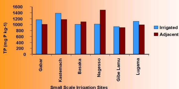
Fig. 2. Status of total phosphorus in irrigated and their adjacent non-irrigated farmlands
