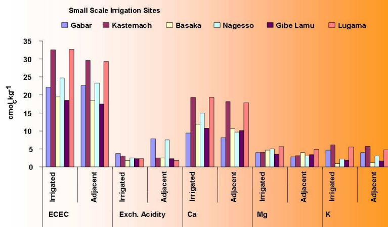
Fig. 4. Exchangeable bases, ECEC and acidity in irrigated and their adjacent non-irrigated farmlands
